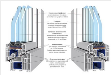
Profile system Salamander bluEvolution
